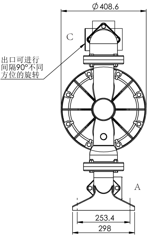
SIDE VIEW 侧视图
